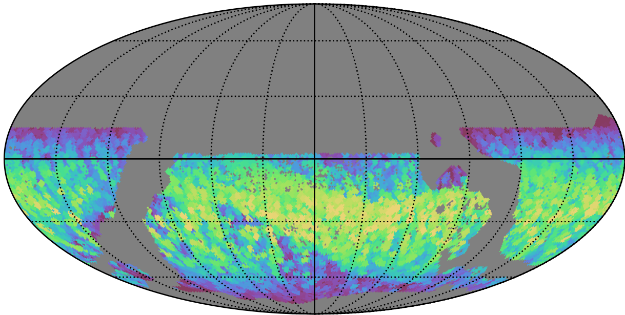
mw_roll_bulge_v3.3_10yrs WFD all bands: Max normairmass
