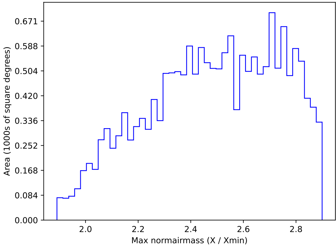
mw_roll_bulge_v3.3_10yrs WFD all bands: Max normairmass
