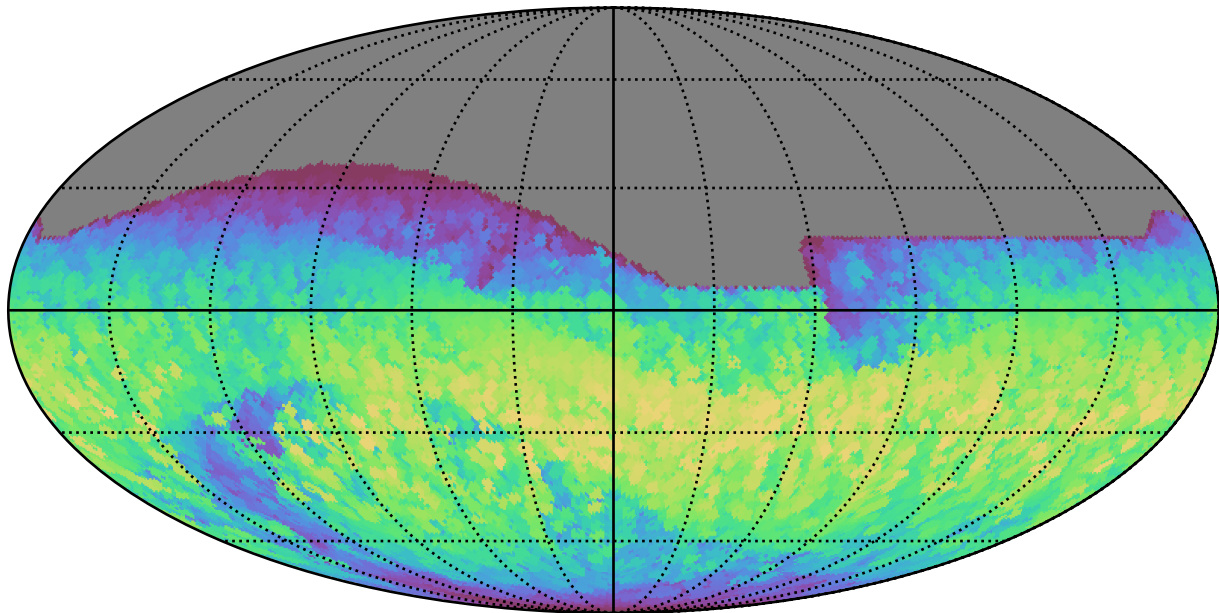
mw_roll_bulge_v3.3_10yrs All sky all bands: Max normairmass
