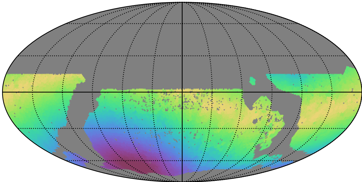
mw_roll_bulge_v3.3_10yrs WFD u band: Max moonDistance
