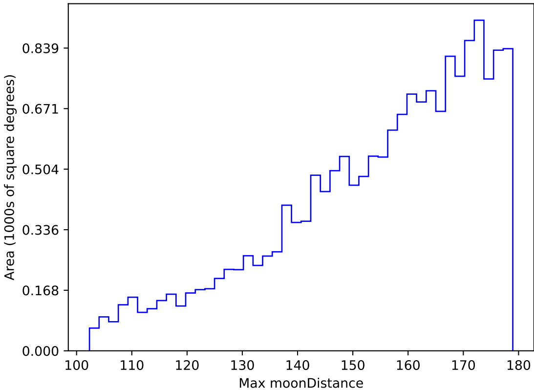
mw_roll_bulge_v3.3_10yrs WFD u band: Max moonDistance
