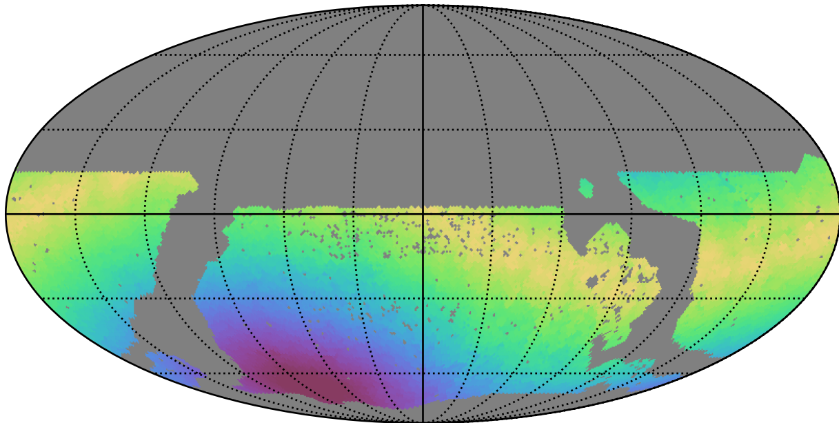
mw_roll_bulge_v3.3_10yrs WFD g band: Max moonDistance
