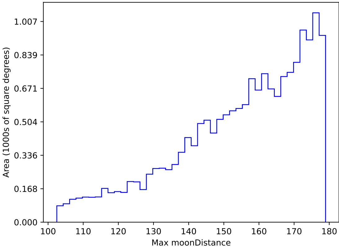
mw_roll_bulge_v3.3_10yrs WFD g band: Max moonDistance
