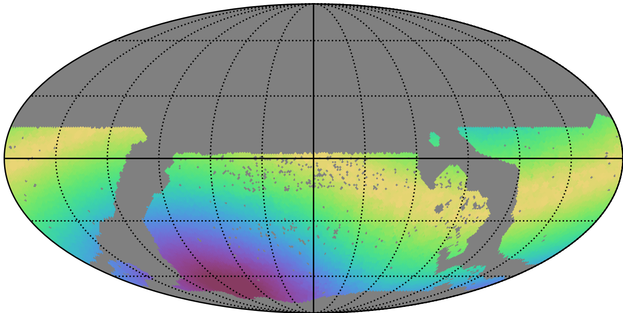
mw_roll_bulge_v3.3_10yrs WFD all bands: Max moonDistance
