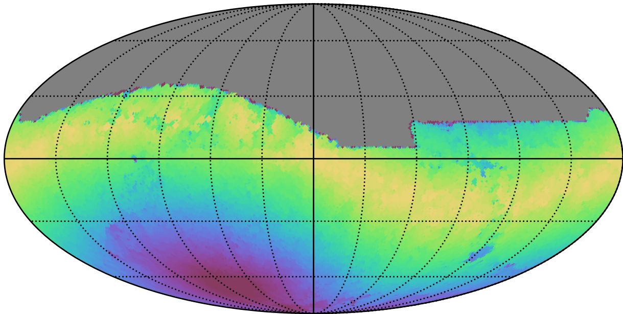
mw_roll_bulge_v3.3_10yrs All sky z band: Max moonDistance
