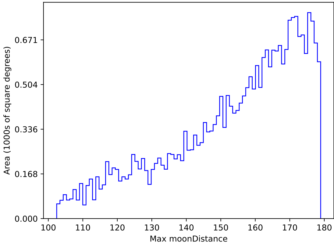
mw_roll_bulge_v3.3_10yrs All sky z band: Max moonDistance
