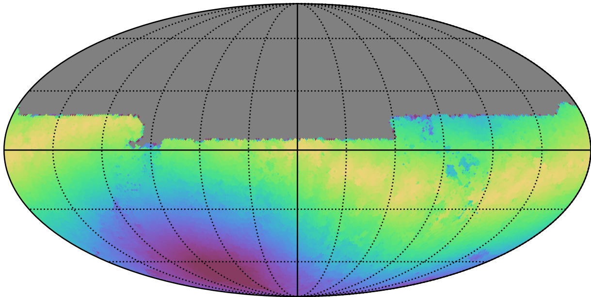
mw_roll_bulge_v3.3_10yrs All sky u band: Max moonDistance
