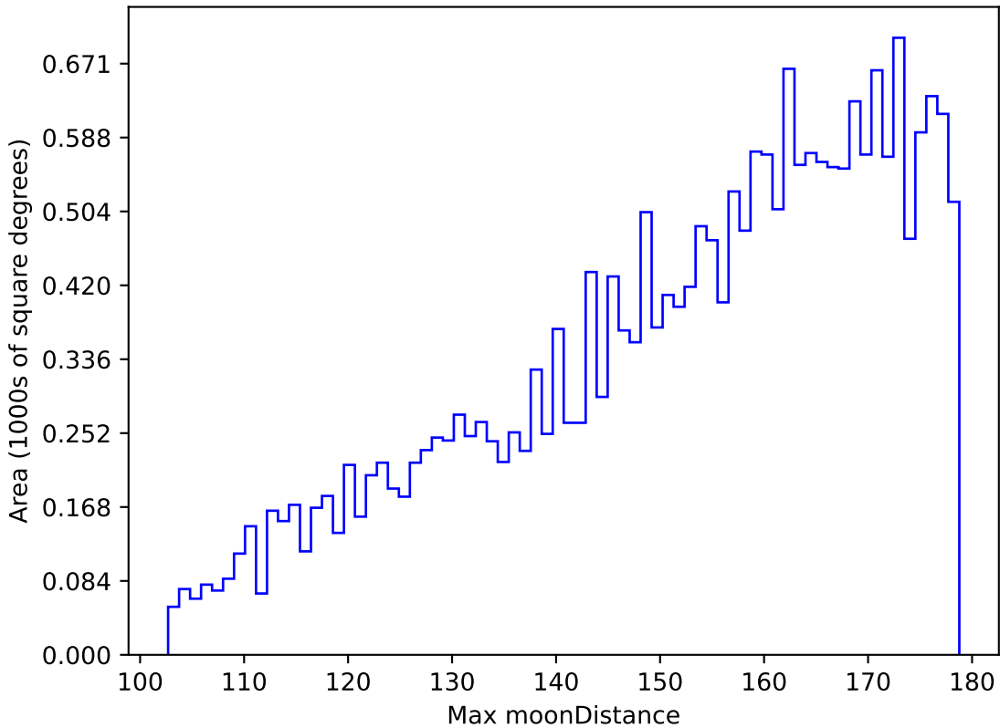
mw_roll_bulge_v3.3_10yrs All sky u band: Max moonDistance
