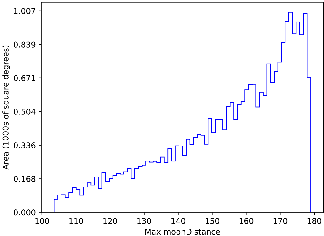
mw_roll_bulge_v3.3_10yrs All sky g band: Max moonDistance
