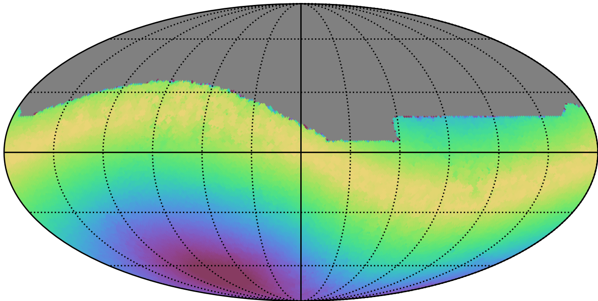
mw_roll_bulge_v3.3_10yrs All sky all bands: Max moonDistance
