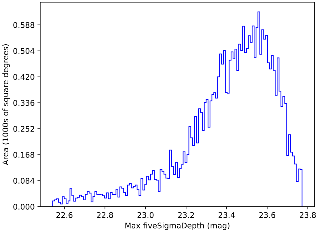
mw_roll_bulge_v3.3_10yrs Yr 1 z band: Max fiveSigmaDepth
