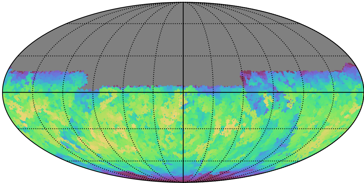
mw_roll_bulge_v3.3_10yrs Yr 1 y band: Max fiveSigmaDepth
