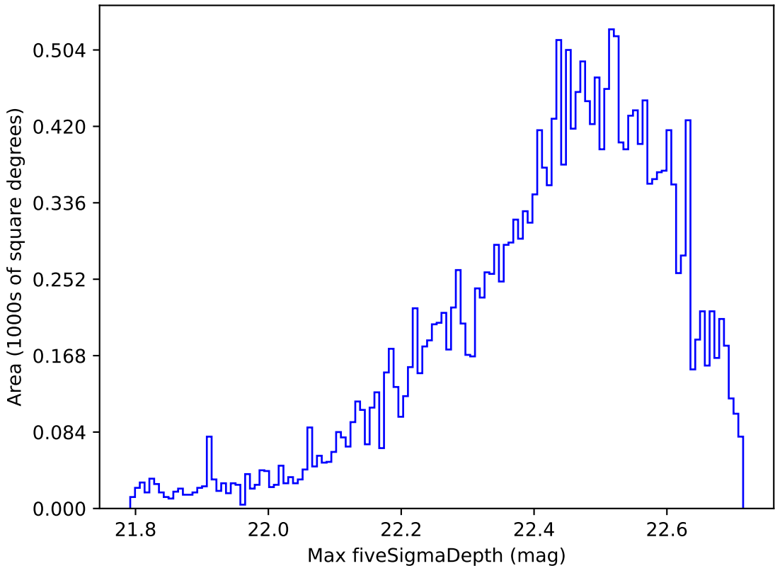
mw_roll_bulge_v3.3_10yrs Yr 1 y band: Max fiveSigmaDepth
