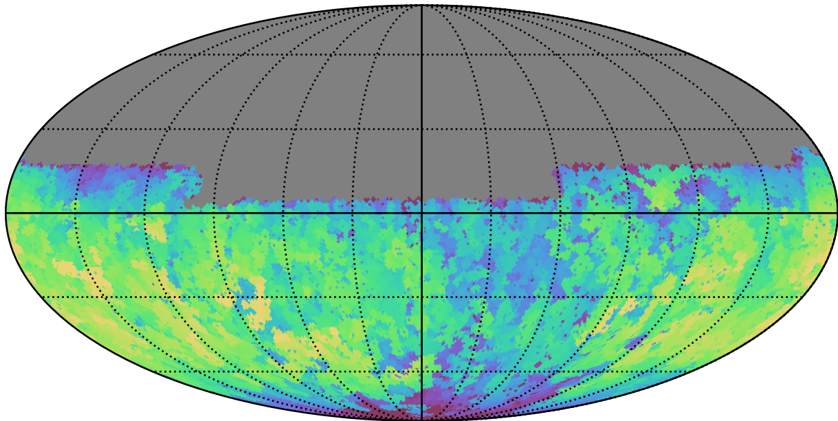
mw_roll_bulge_v3.3_10yrs Yr 1 u band: Max fiveSigmaDepth
