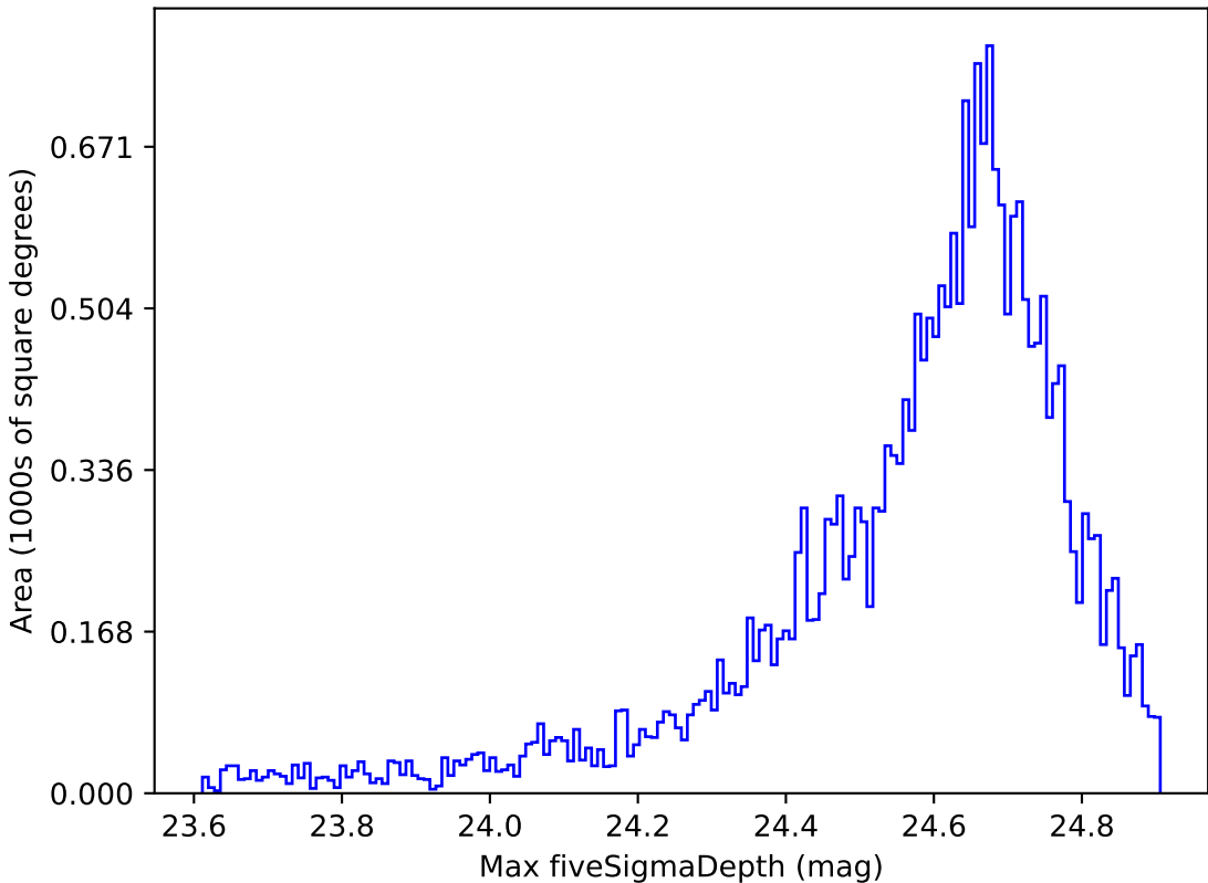
mw_roll_bulge_v3.3_10yrs Yr 1 r band: Max fiveSigmaDepth
