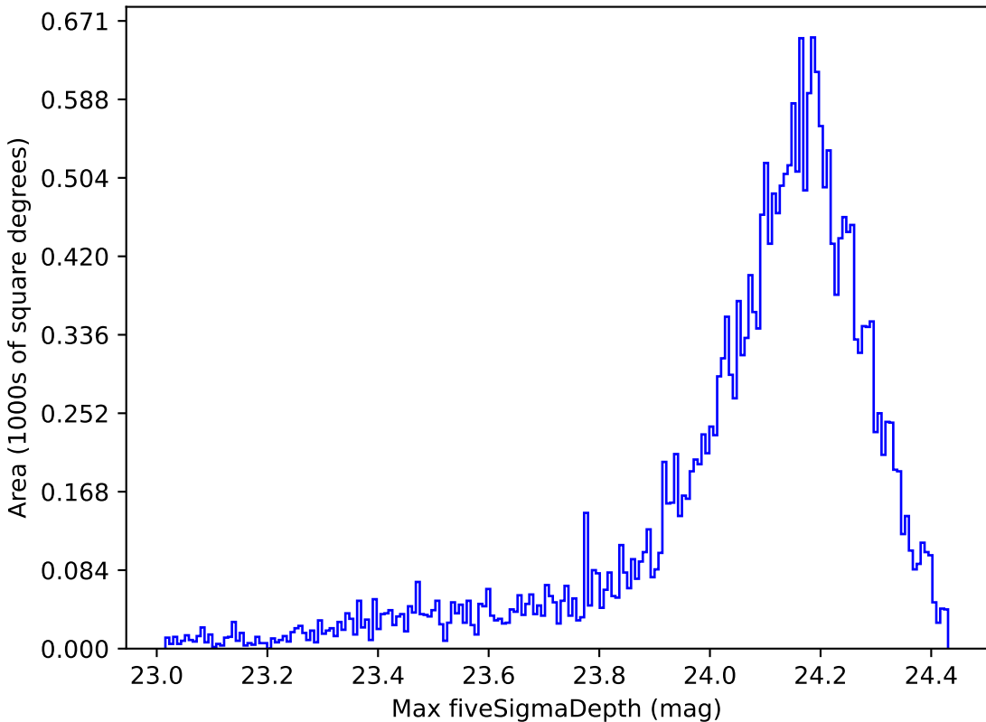
mw_roll_bulge_v3.3_10yrs Yr 1 i band: Max fiveSigmaDepth
