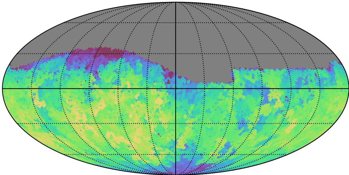
mw_roll_bulge_v3.3_10yrs Yr 1 g band: Max fiveSigmaDepth
