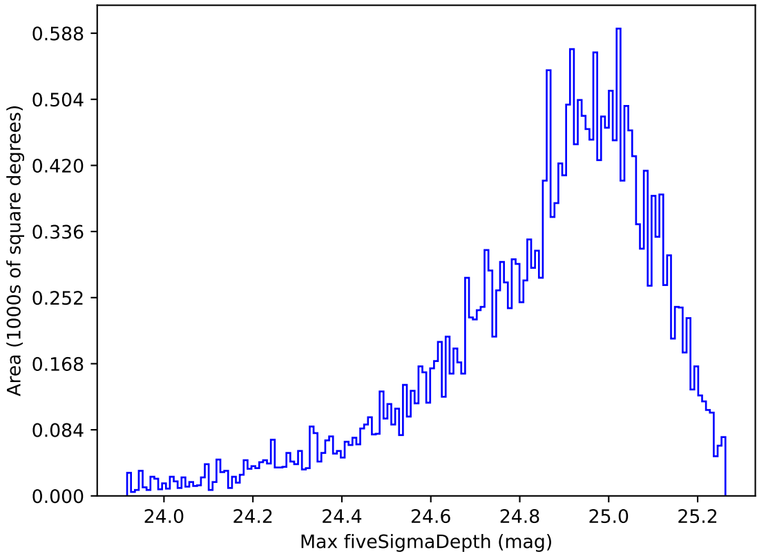
mw_roll_bulge_v3.3_10yrs Yr 1 g band: Max fiveSigmaDepth
