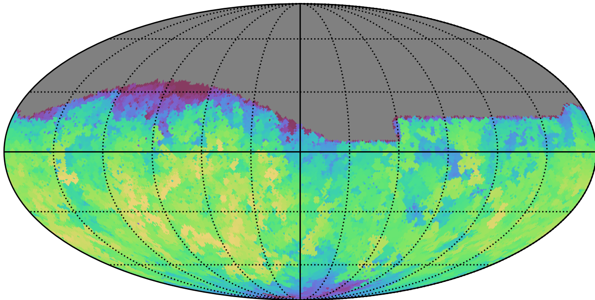
mw_roll_bulge_v3.3_10yrs Yr 1 all bands: Max fiveSigmaDepth
