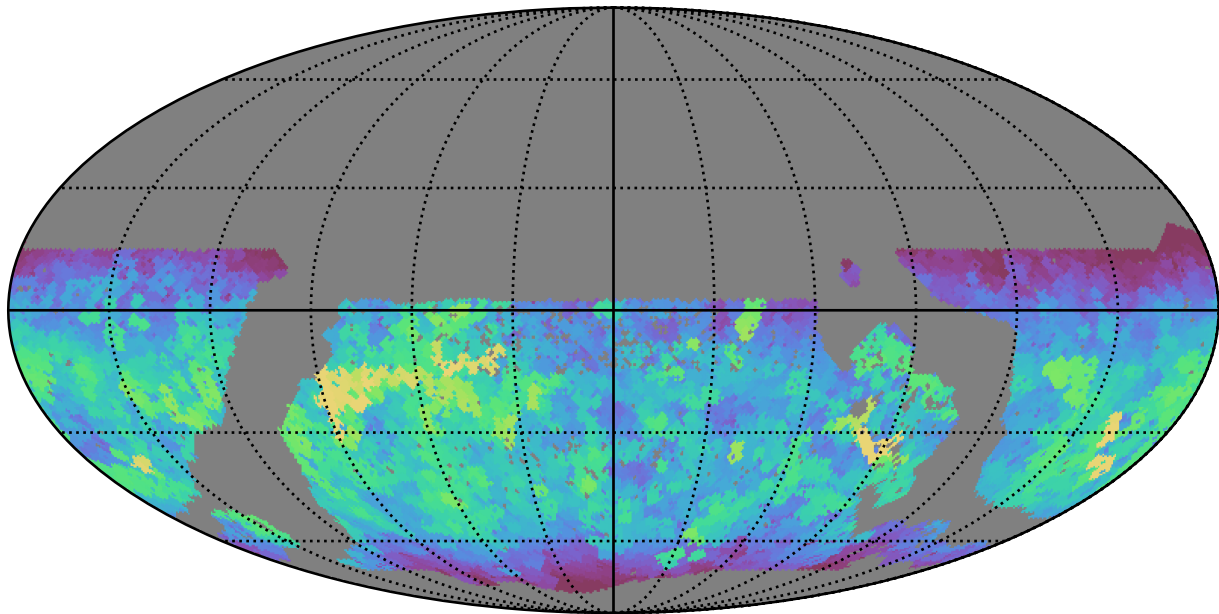
mw_roll_bulge_v3.3_10yrs WFD z band: Max fiveSigmaDepth
