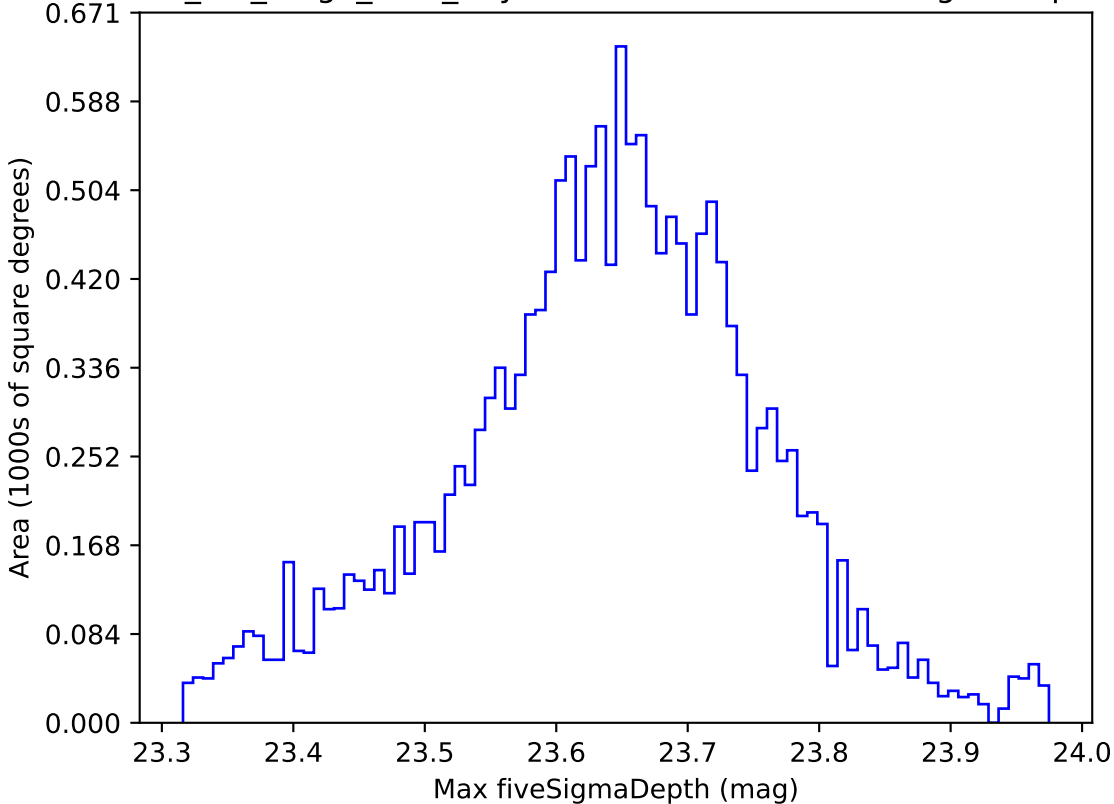
mw_roll_bulge_v3.3_10yrs WFD z band: Max fiveSigmaDepth
