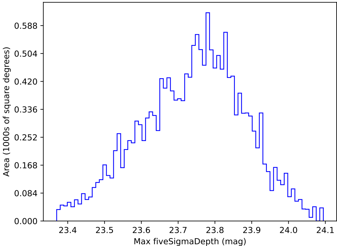
mw_roll_bulge_v3.3_10yrs WFD u band: Max fiveSigmaDepth
