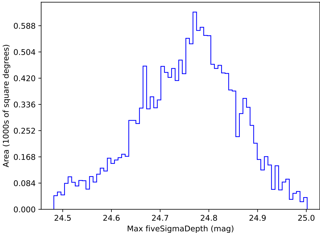
mw_roll_bulge_v3.3_10yrs WFD r band: Max fiveSigmaDepth
