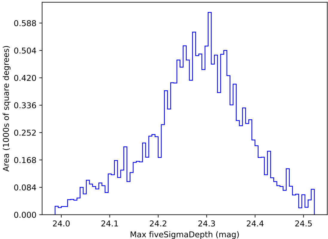
mw_roll_bulge_v3.3_10yrs WFD i band: Max fiveSigmaDepth
