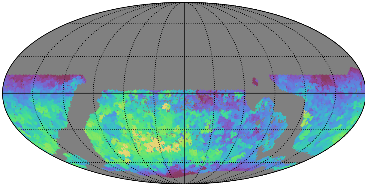
mw_roll_bulge_v3.3_10yrs WFD g band: Max fiveSigmaDepth
