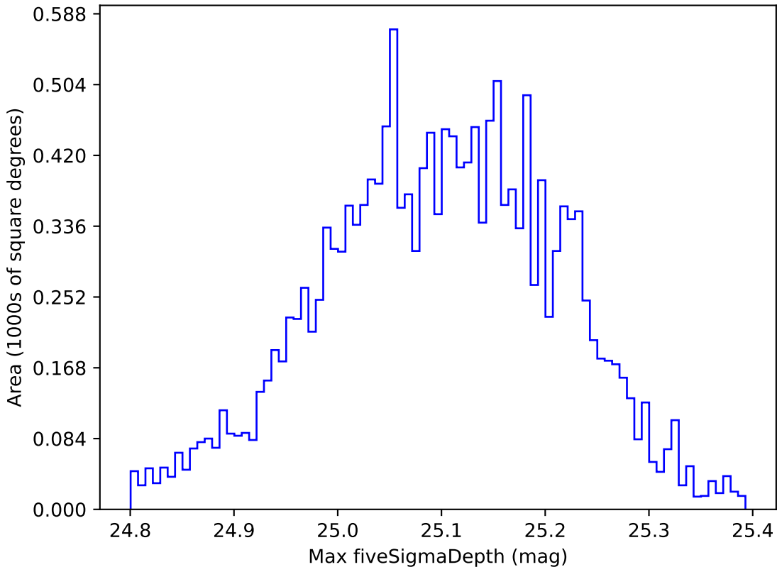
mw_roll_bulge_v3.3_10yrs WFD g band: Max fiveSigmaDepth
