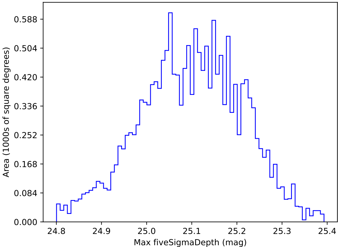
mw_roll_bulge_v3.3_10yrs WFD all bands: Max fiveSigmaDepth
