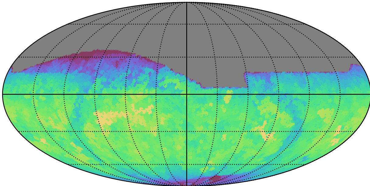
mw_roll_bulge_v3.3_10yrs All sky z band: Max fiveSigmaDepth
