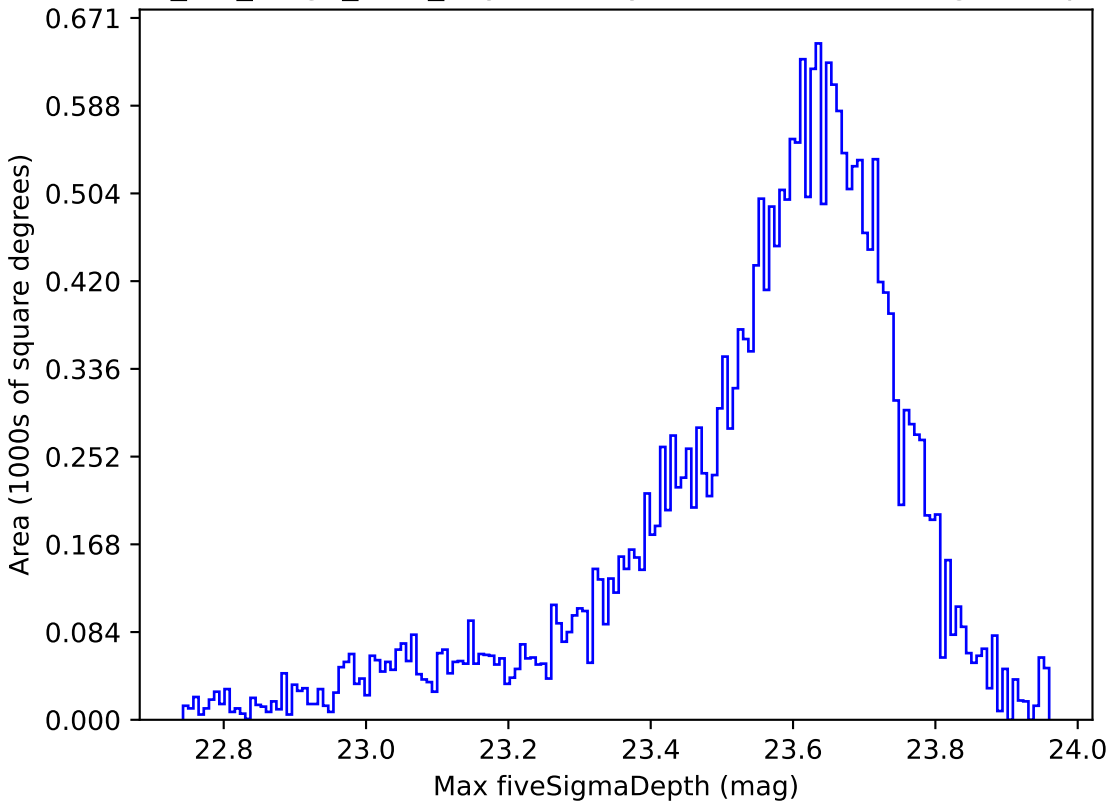
mw_roll_bulge_v3.3_10yrs All sky z band: Max fiveSigmaDepth
