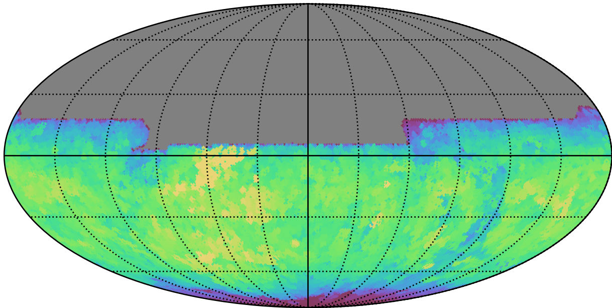
mw_roll_bulge_v3.3_10yrs All sky y band: Max fiveSigmaDepth
