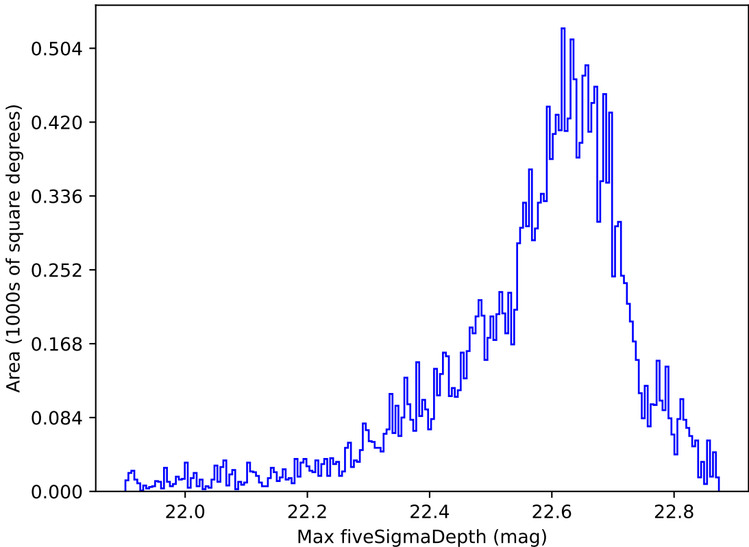
mw_roll_bulge_v3.3_10yrs All sky y band: Max fiveSigmaDepth
