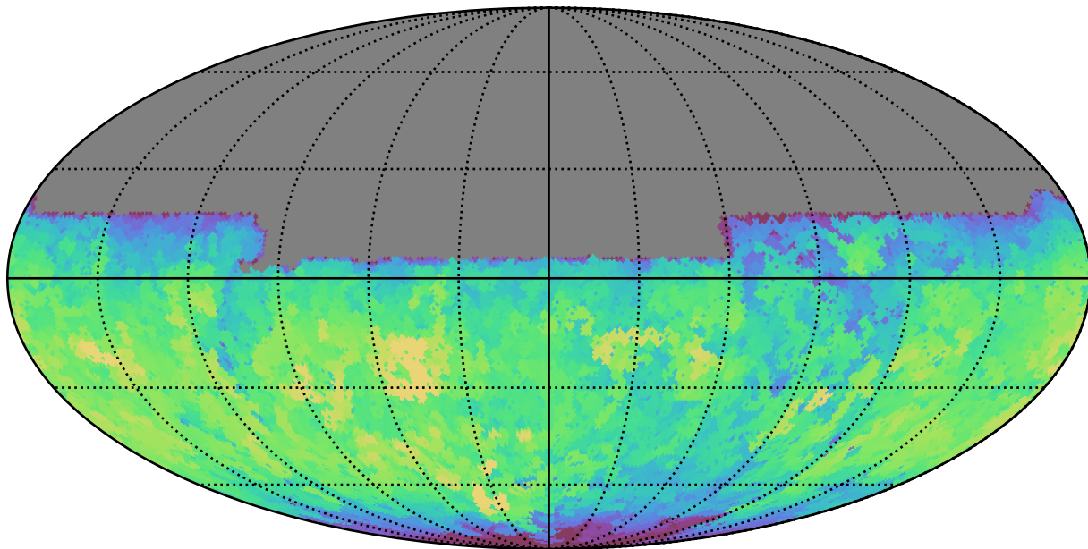
mw_roll_bulge_v3.3_10yrs All sky u band: Max fiveSigmaDepth
