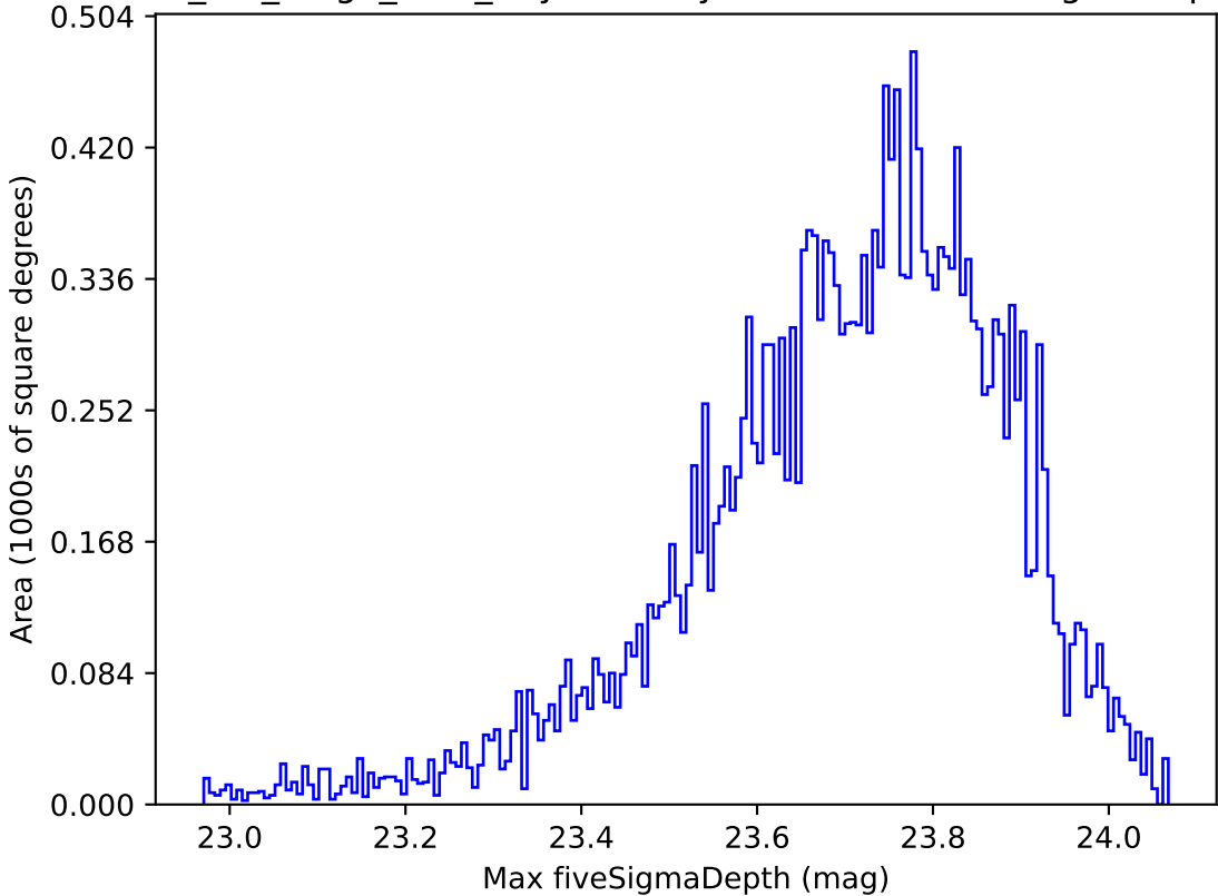
mw_roll_bulge_v3.3_10yrs All sky u band: Max fiveSigmaDepth
