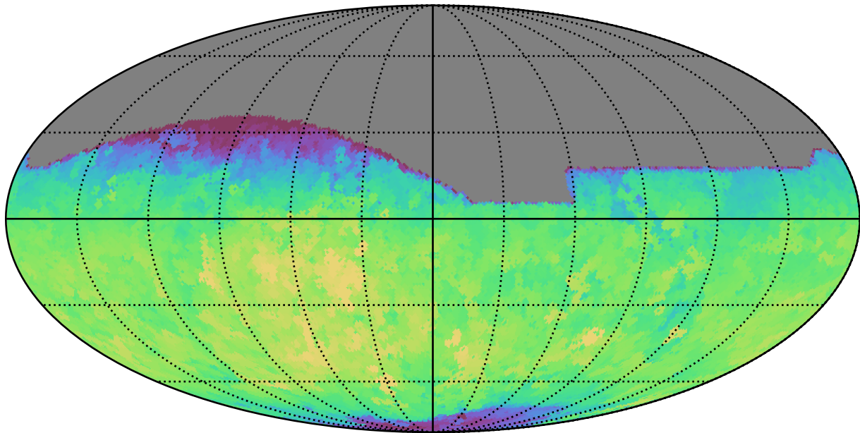
mw_roll_bulge_v3.3_10yrs All sky r band: Max fiveSigmaDepth
