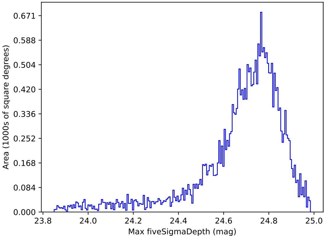
mw_roll_bulge_v3.3_10yrs All sky r band: Max fiveSigmaDepth
