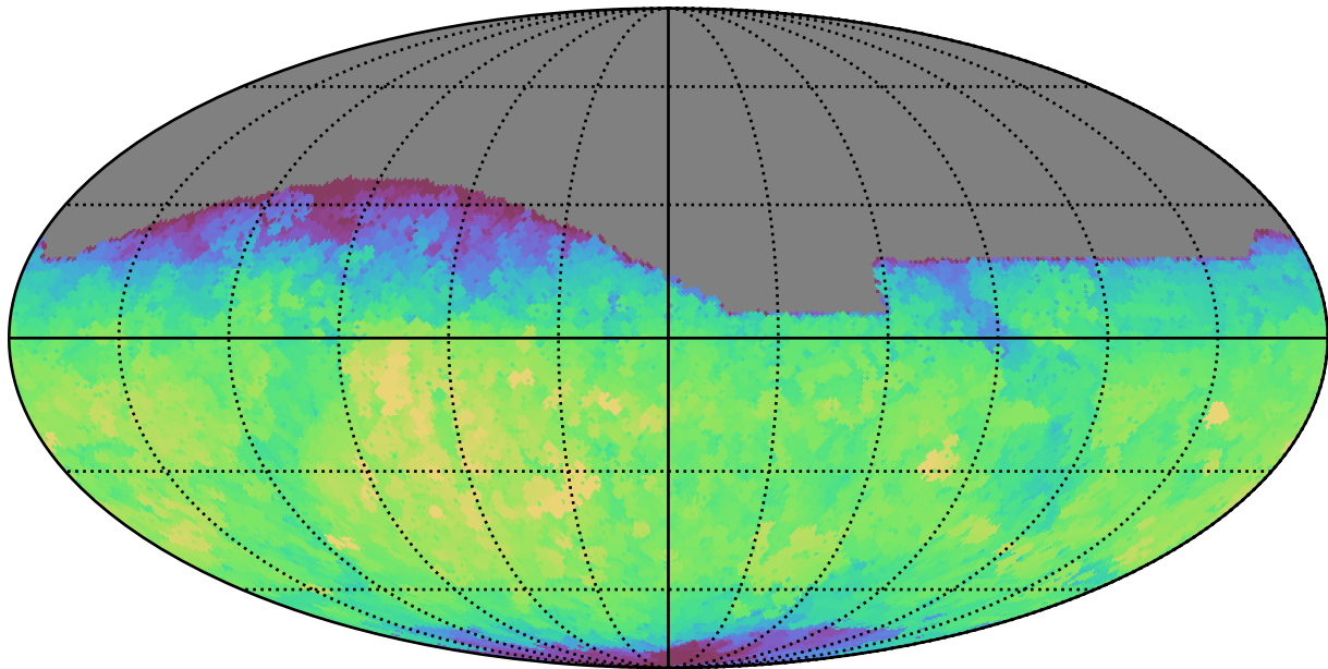
mw_roll_bulge_v3.3_10yrs All sky i band: Max fiveSigmaDepth
