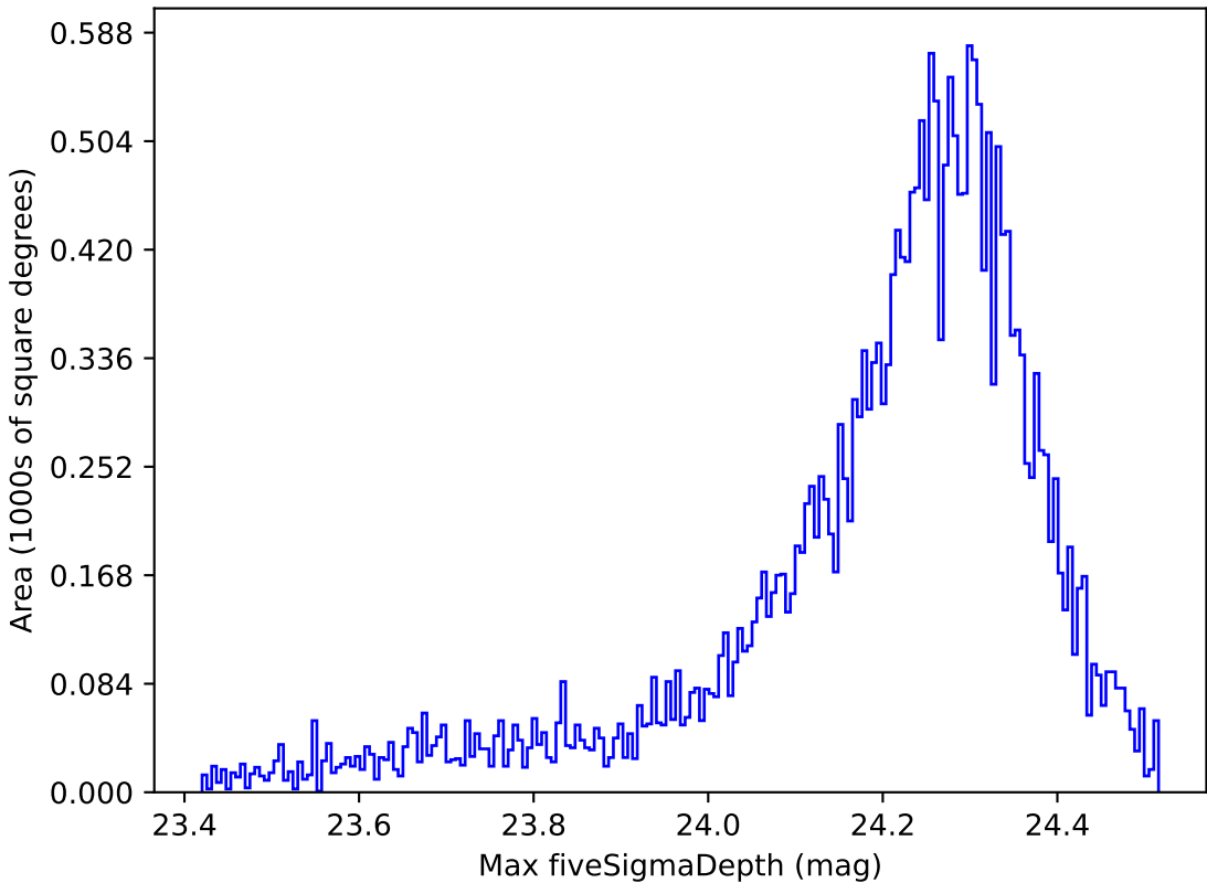
mw_roll_bulge_v3.3_10yrs All sky i band: Max fiveSigmaDepth
