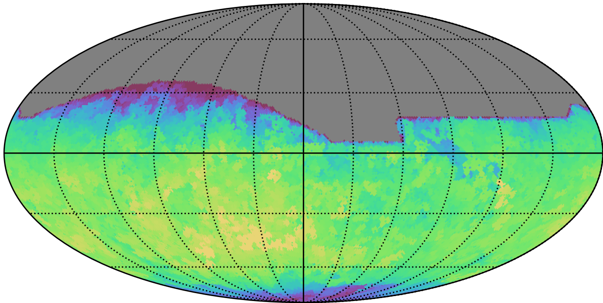
mw_roll_bulge_v3.3_10yrs All sky all bands: Max fiveSigmaDepth
