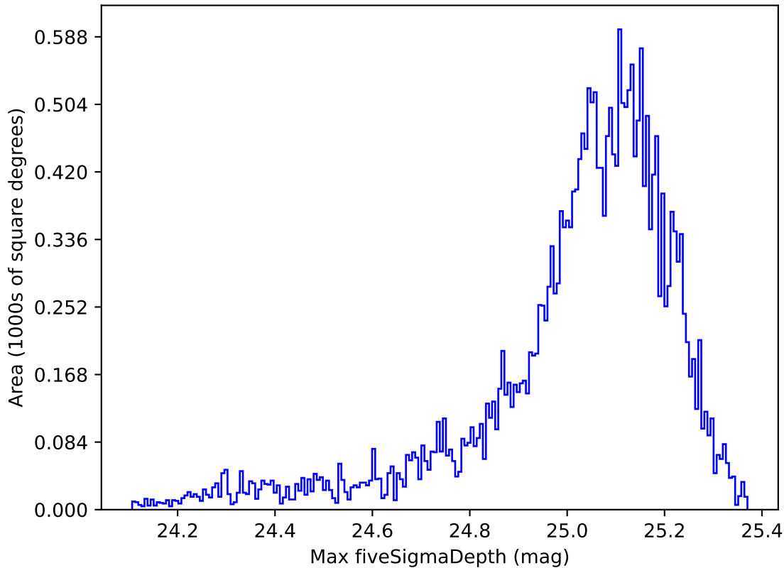
mw_roll_bulge_v3.3_10yrs All sky all bands: Max fiveSigmaDepth
