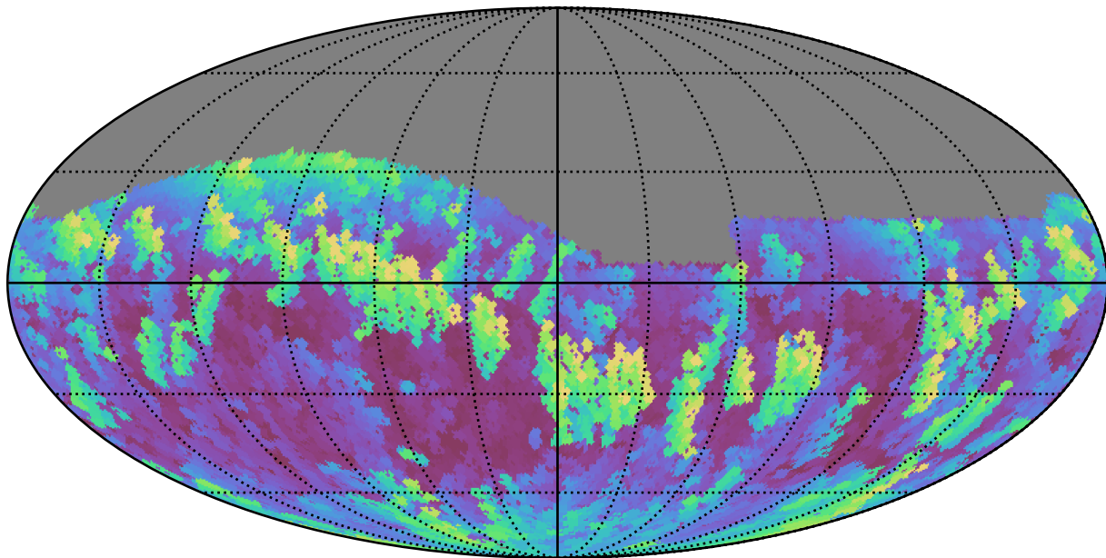
mw_roll_bulge_v3.3_10yrs Yr 1 z band: Max airmass
