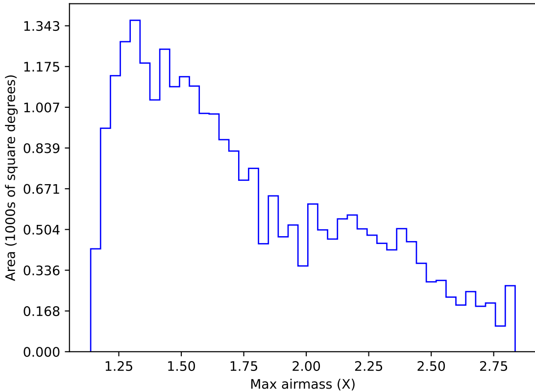
mw_roll_bulge_v3.3_10yrs Yr 1 z band: Max airmass
