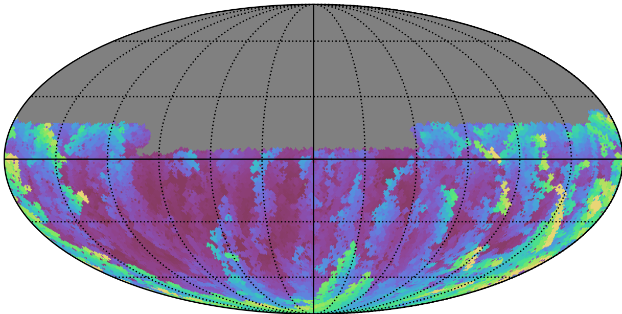
mw_roll_bulge_v3.3_10yrs Yr 1 u band: Max airmass
