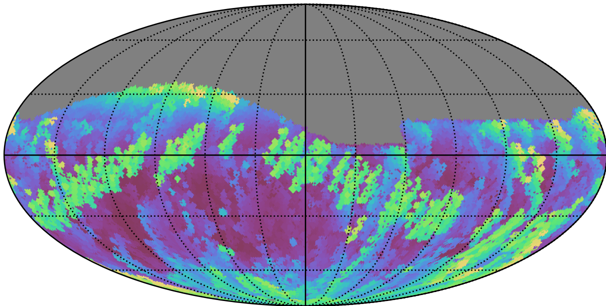
mw_roll_bulge_v3.3_10yrs Yr 1 r band: Max airmass
