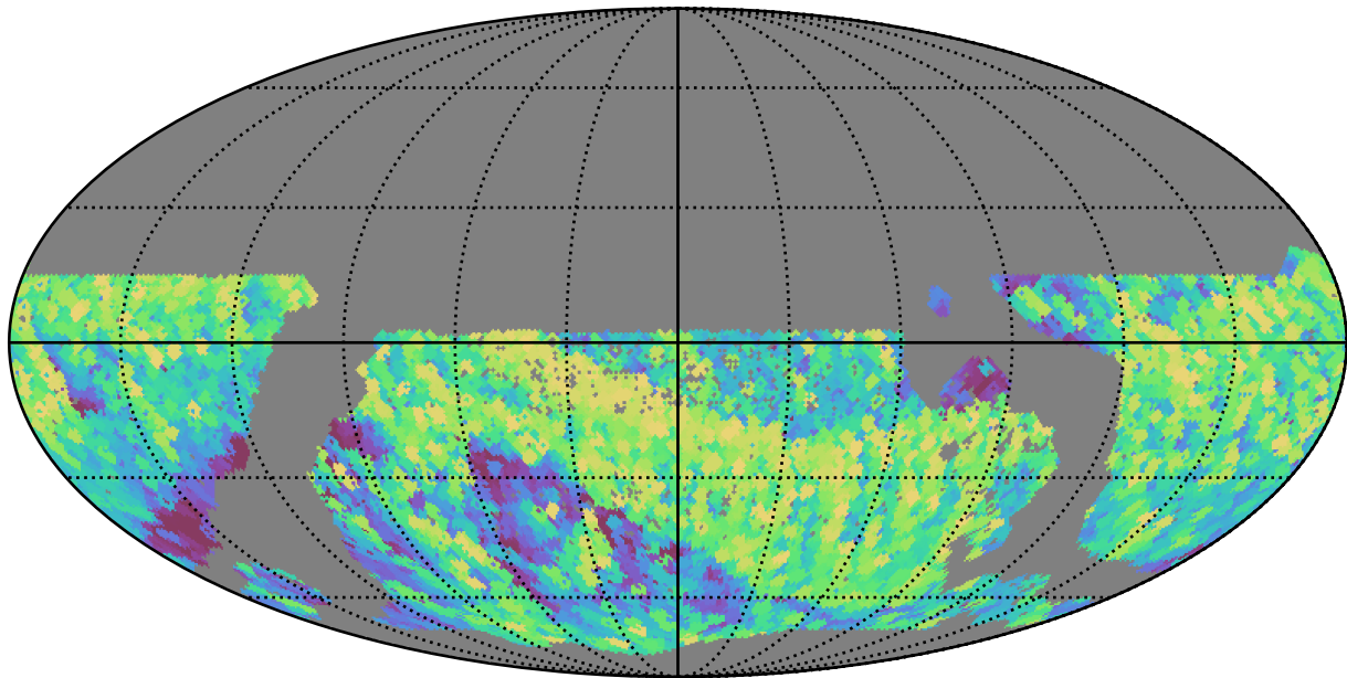
mw_roll_bulge_v3.3_10yrs WFD z band: Max airmass
