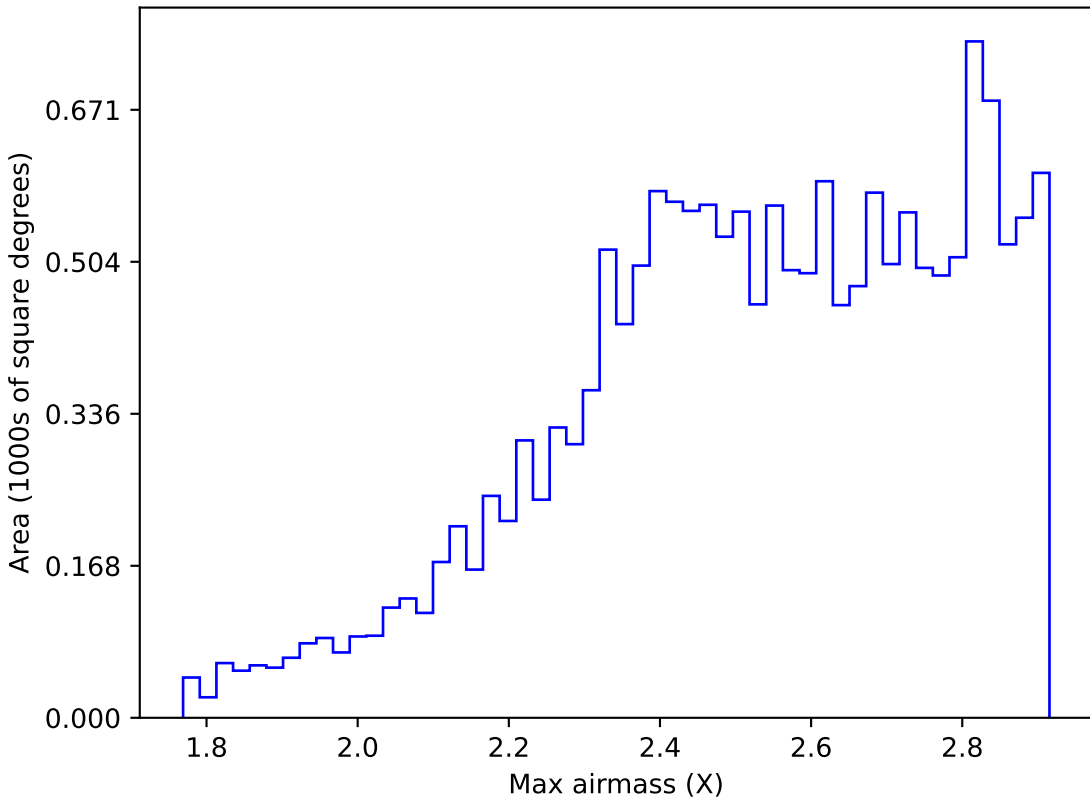
mw_roll_bulge_v3.3_10yrs WFD z band: Max airmass
