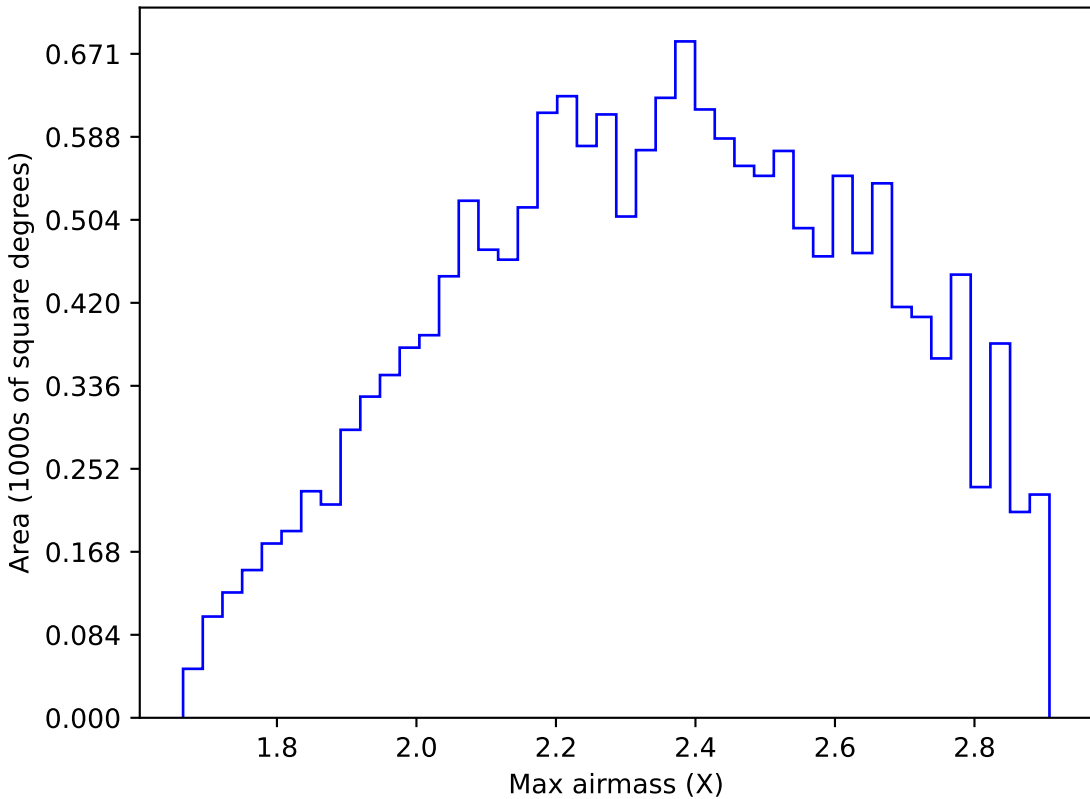
mw_roll_bulge_v3.3_10yrs WFD y band: Max airmass
